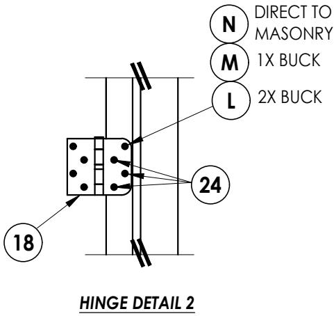
HINGE DETAIL 2
